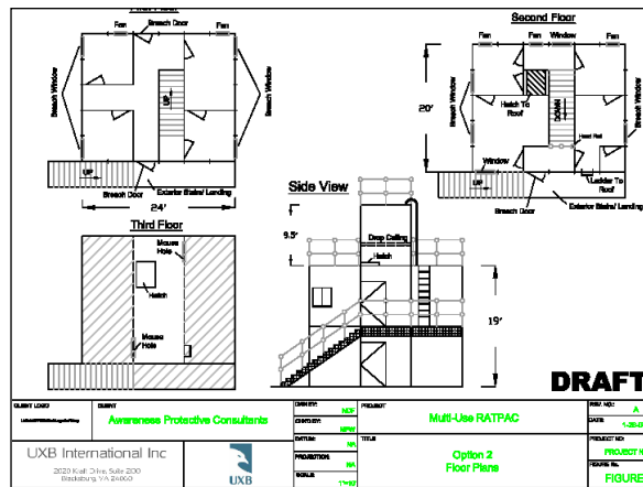
RATPAC can be easily reconfigured to various floor plans to keep the training fresh and to fit specific needs.
